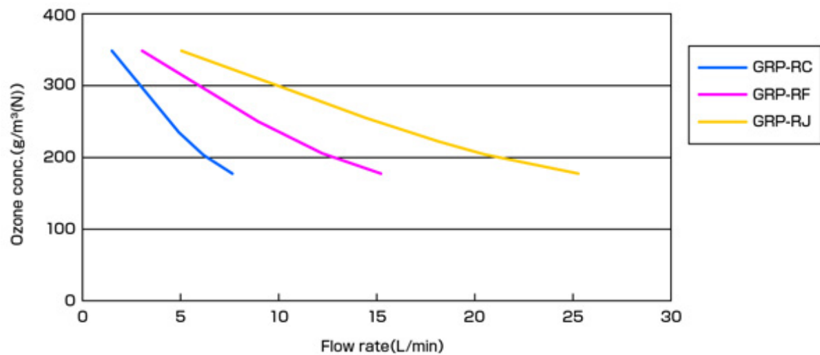
GRP series performance curve
