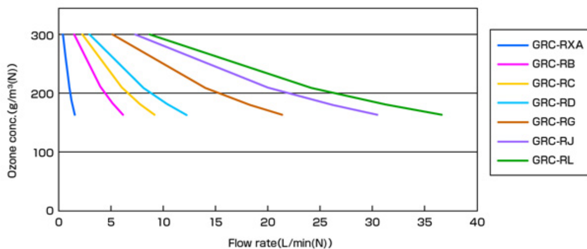
GRC series performance curve
