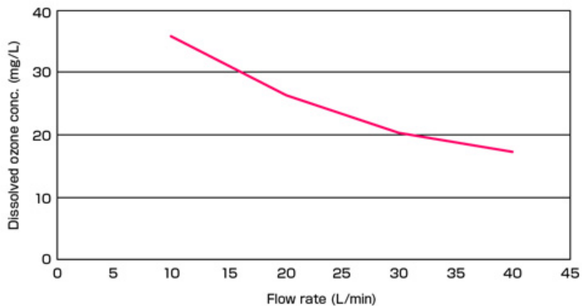
Ozonized water performance curve
