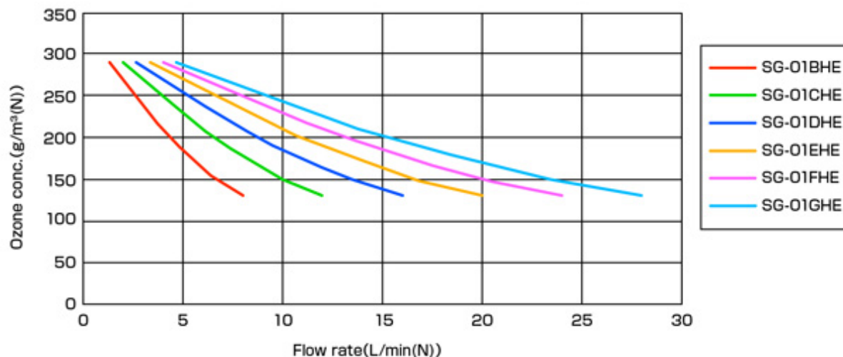
SG-HE series performance curve
