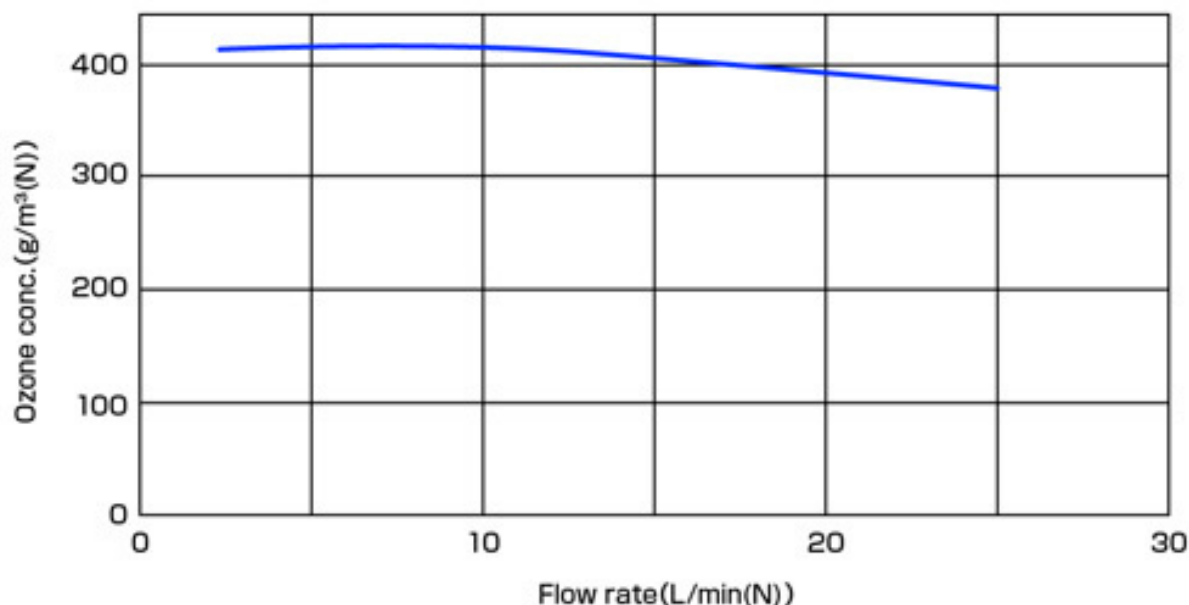
SGRF-03JA Performance curve
