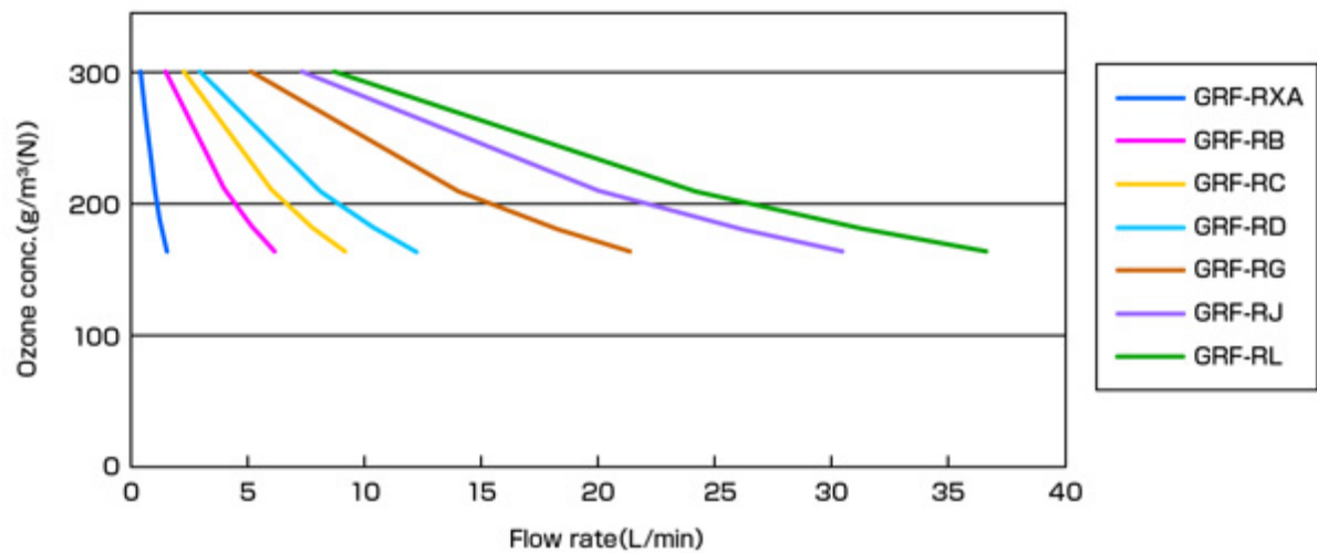
GRF series performance curve
